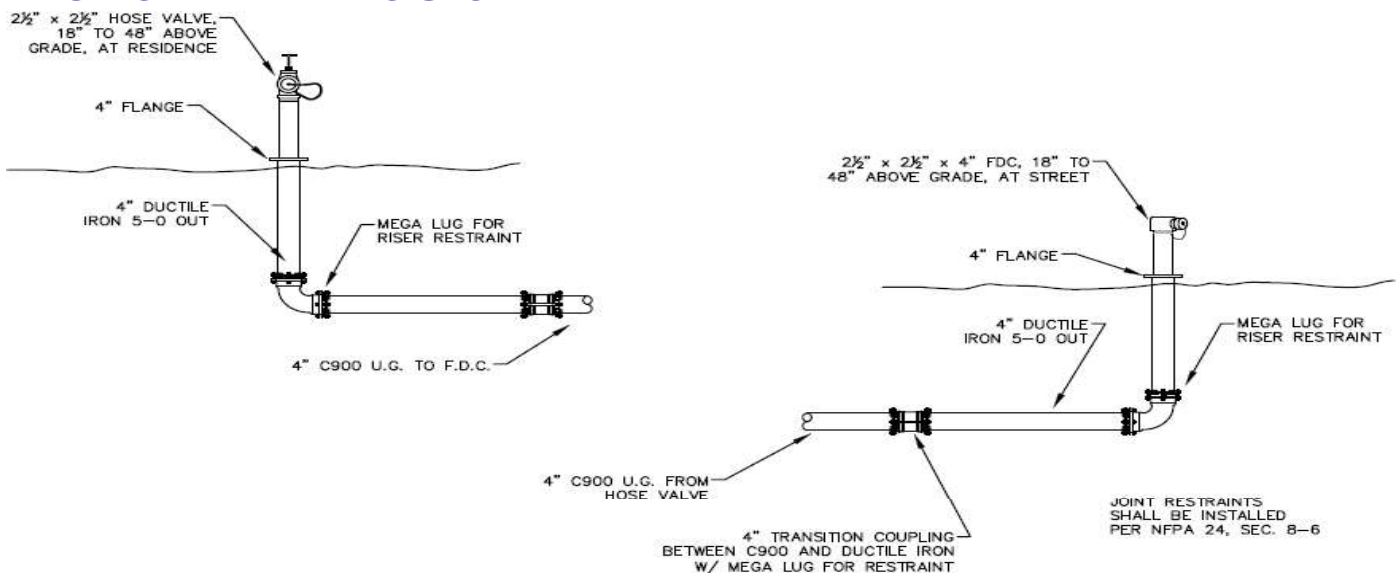
DRY STANDPIPE DETAIL
